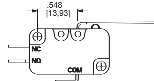
LOW FORCE, HIGH MOTION PIVOT POSITION
