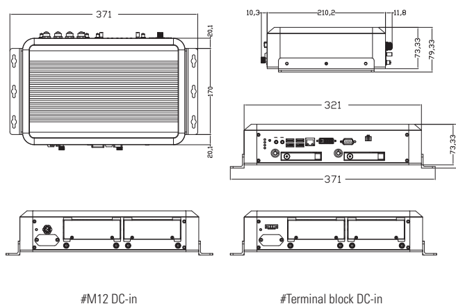
#M12 DC-in
