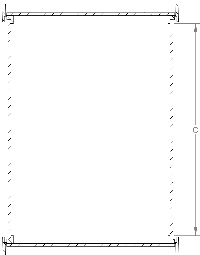
SECTION B-B
