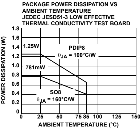
FIGURE 8. PACKAGE POWER DISSIPATION vs AMBIENT TEMPERATURE
