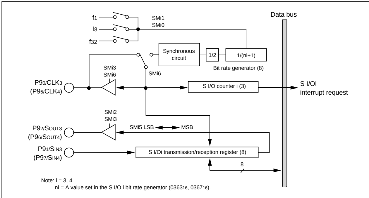
Figure 1.16.31. S I/O3, 4 block diagram
