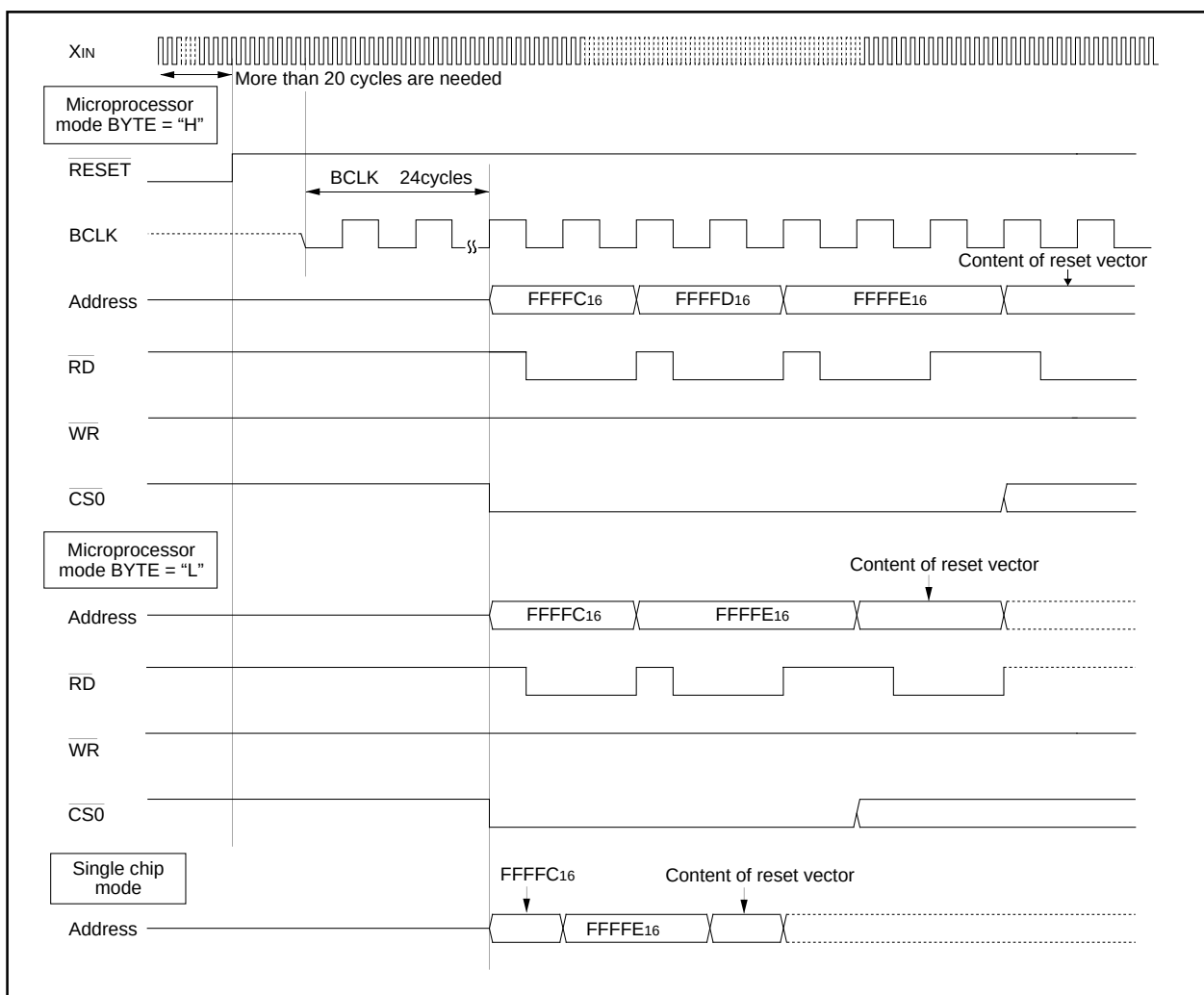
Figure 1.5.2. Reset sequence
