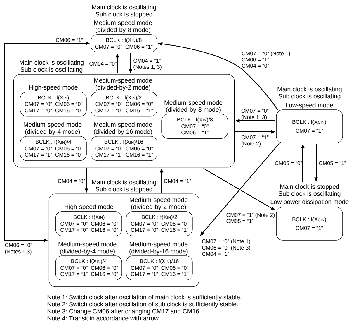
Figure 2.15.1. State transition diagram of power control mode
