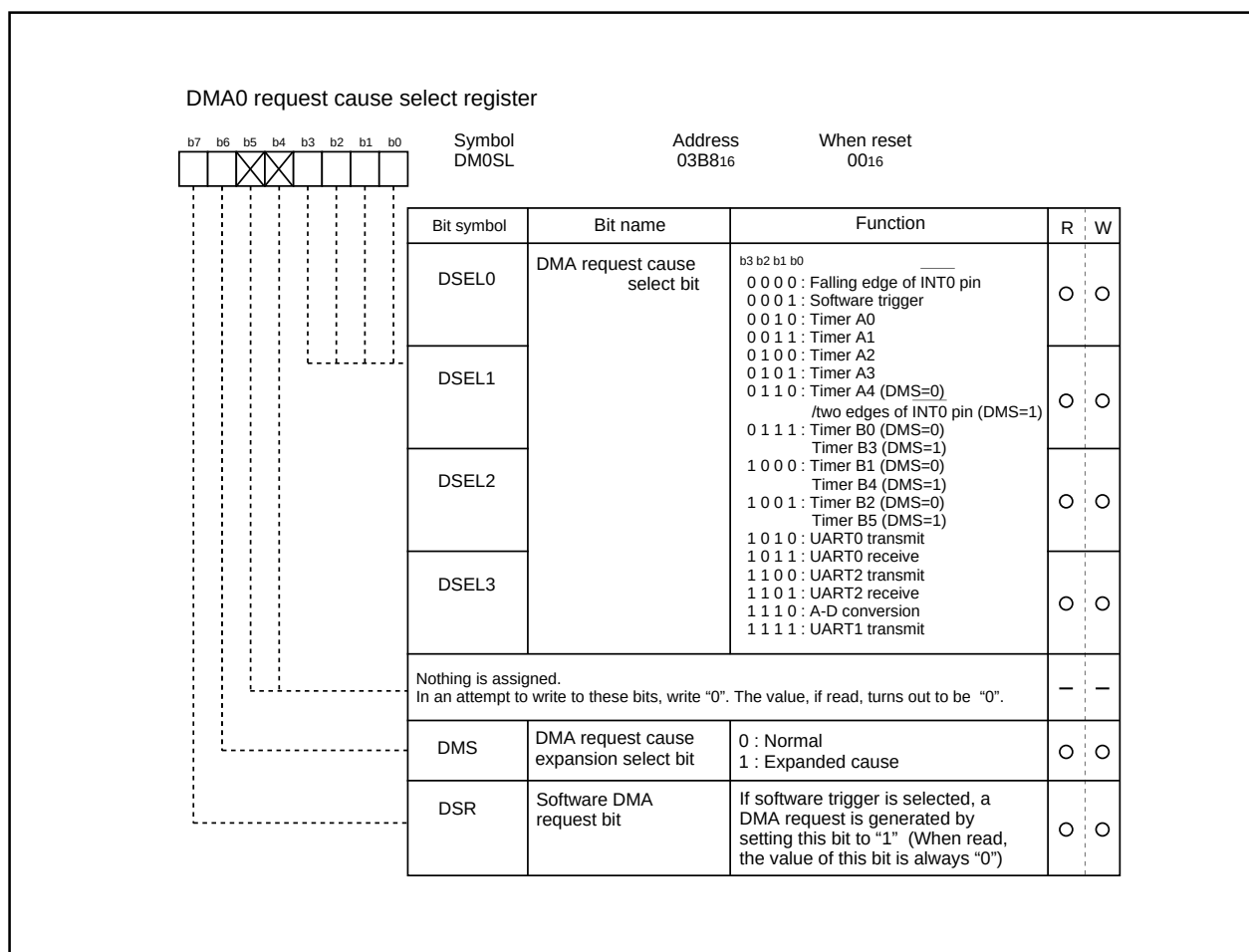
Figure 1.13.2. DMAC register (1)
