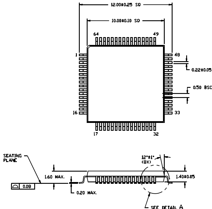
64-Pin Thin Plastic Quad Flat Pack (10 x 10 x 1.4 mm) A64 64-Pin Pb-Free Thin Plastic Quad Flat Pack (10 x 10 x 1.4 mm) A64
