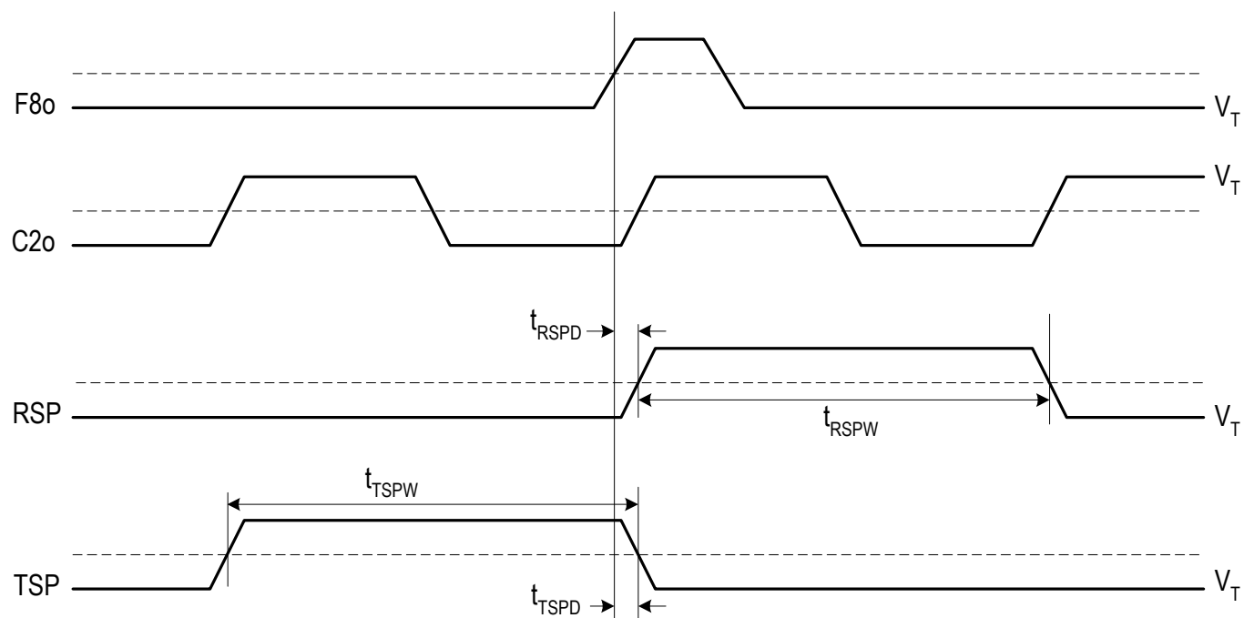
Figure - 13 Output Timing 2
