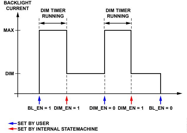
Figure 34. Dim Timer
