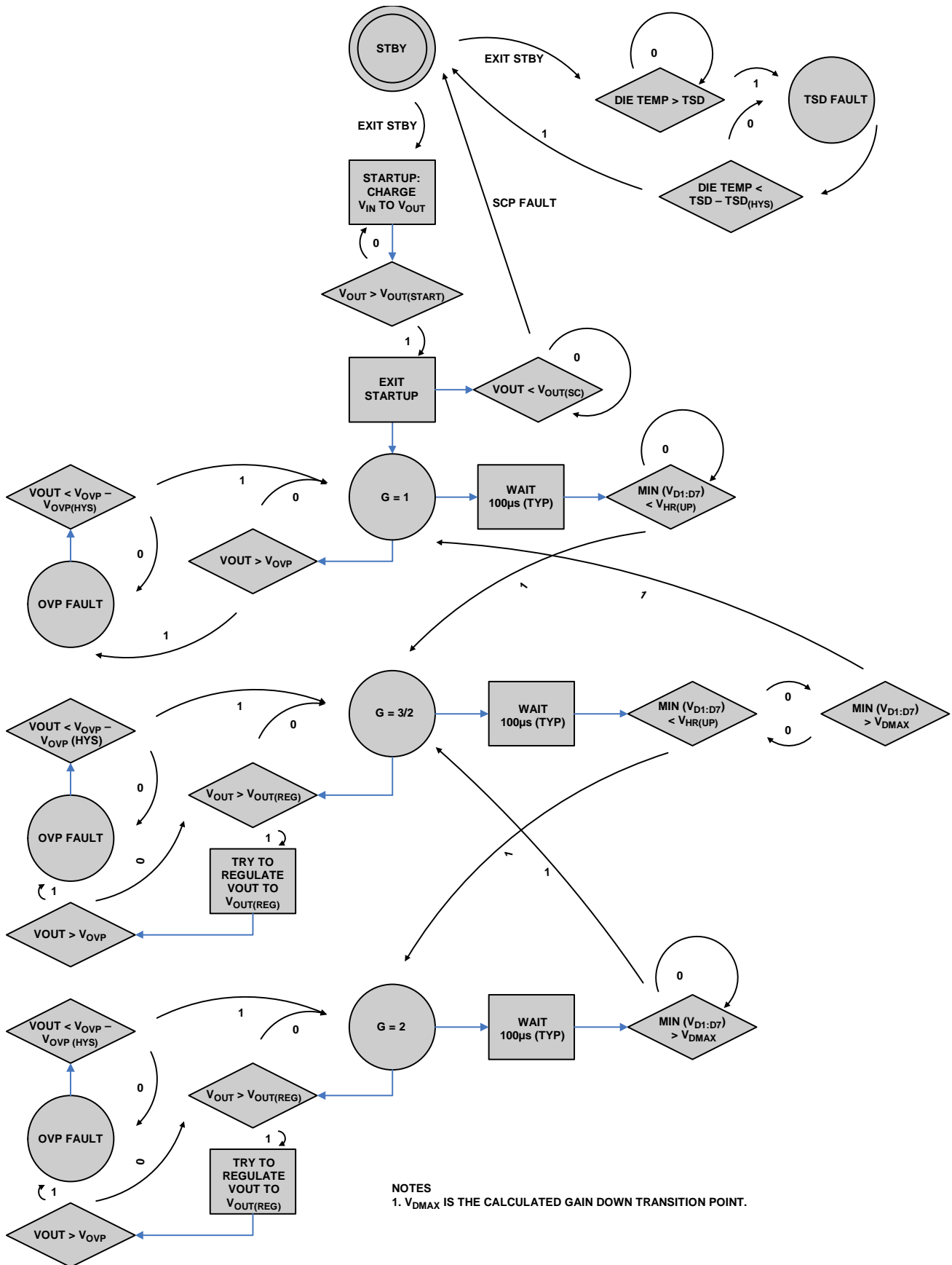
Figure 42. Fault State Machine Rev. A | Page 20 of 48
