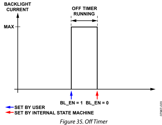
Figure 35. Off Timer
