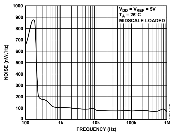
Figure 21. Noise Spectral Density
