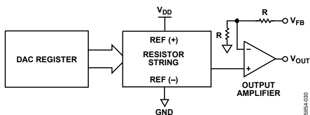
Figure 22. DAC Architecture
