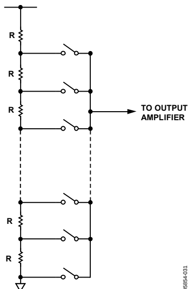
Figure 23. Resistor String
