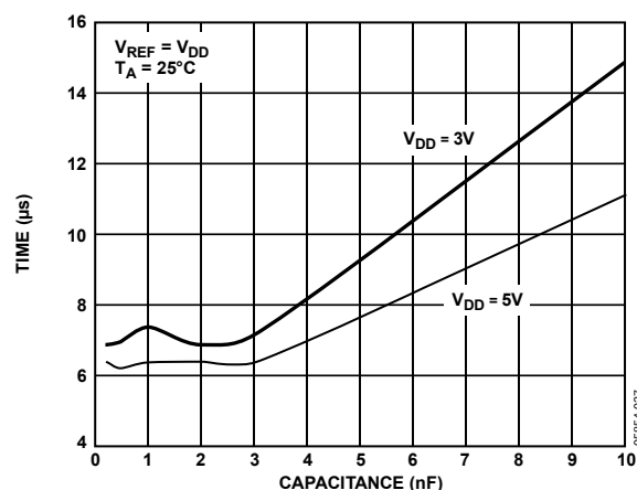
Figure 19. Settling Time vs. Capacitive Load
