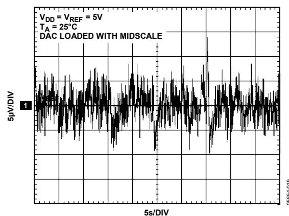
Figure 20. 0.1 Hz to 10 Hz Output Noise Plot
