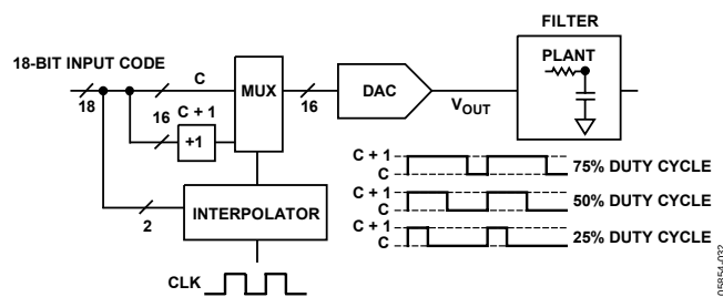
Figure 24. Interpolation Architecture
