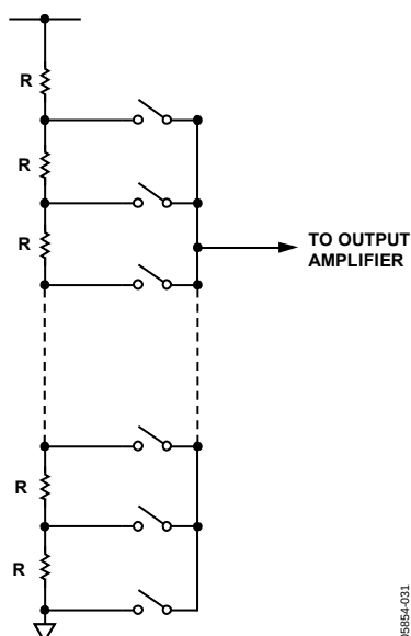
Figure 23. Resistor String
