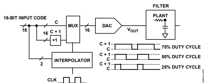
Figure 24. Interpolation Architecture
