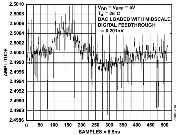
Figure 17. Digital Feedthrough
