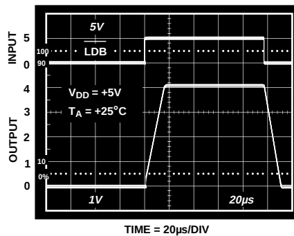
Figure 12. Large Signal Settling Time
