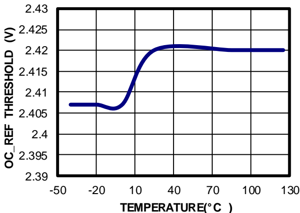
OCREF Threshold vs. Temperature OCREF = 2.4V
