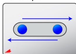
Horizontal Scroll/Pan
