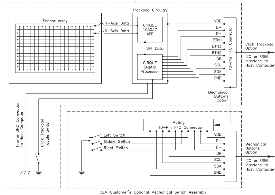
Figure 3. TM105065-2 System Interface Block Diagram
