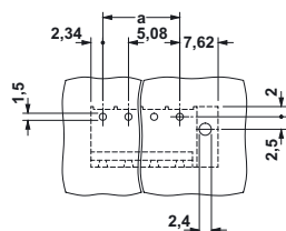
CC 2,5/...-GFR-5,08P26THR
