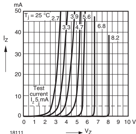
Fig. 12 - Breakdown Characteristics
