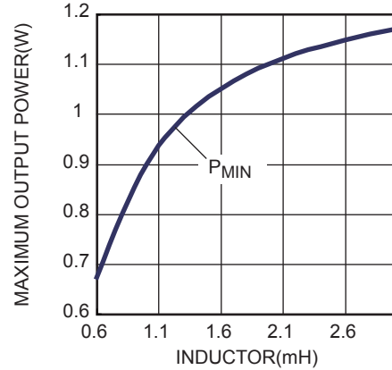
Figure 8: P_{\min} vs. L at 5V
