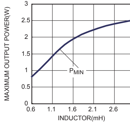
Figure 9: P_{\min} vs. L at 12V
