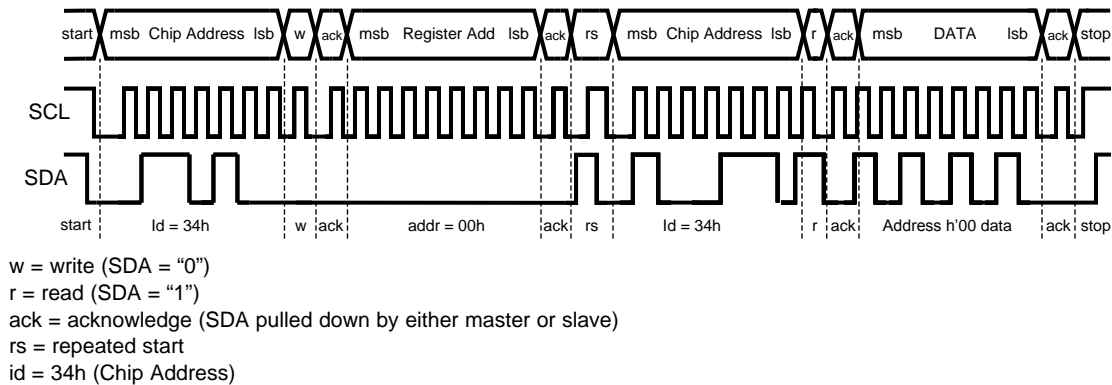
Figure 9. I 2 C DVM Timing for V CC_APPS (Buck1)
