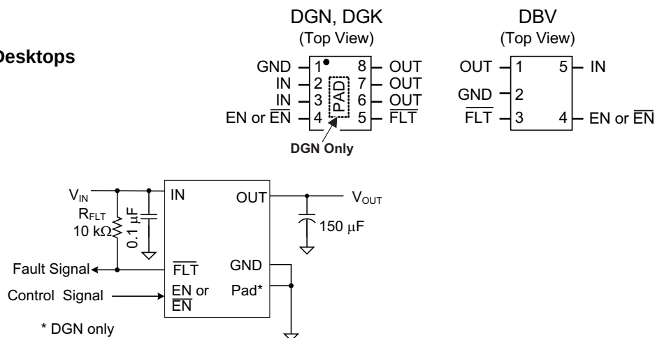
Figure 1. Typical Application
