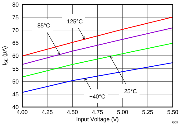
Figure 37. Enabled Supply Current ( I_{SE} ) vs Input Voltage
