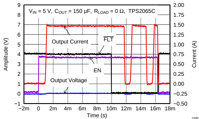
Figure 13. TPS2065C Enable into Output Short
