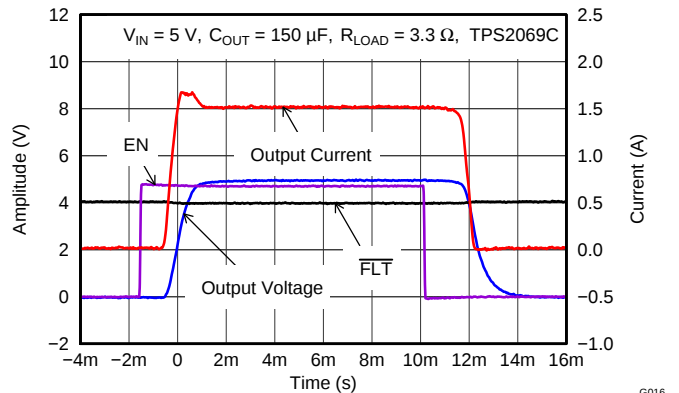
Figure 26. TPS2069C Turn ON into 3.3Ω
