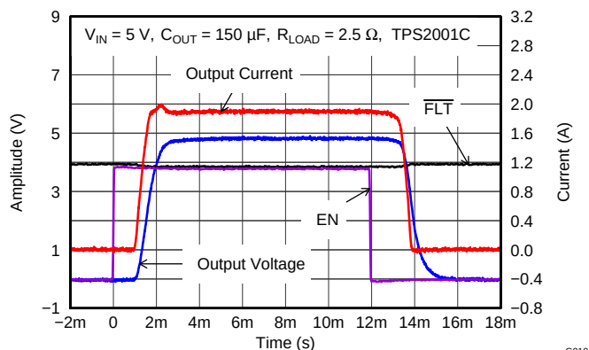
Figure 20. TPS2001C Turn ON into 2.5Ω
