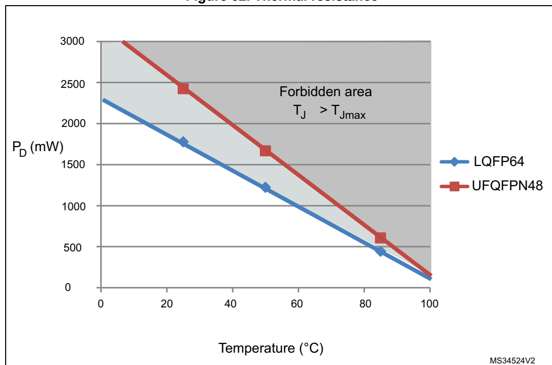
Figure 32. Thermal resistance
