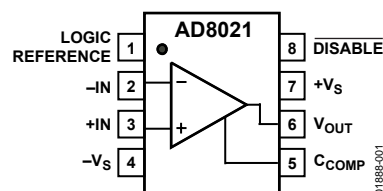
Figure 1. SOIC-8 (R-8) and MSOP-8 (RM-8)
