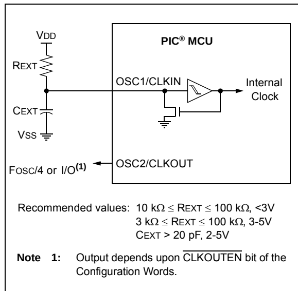
FIGURE 6-6: EXTERNAL RC MODES
