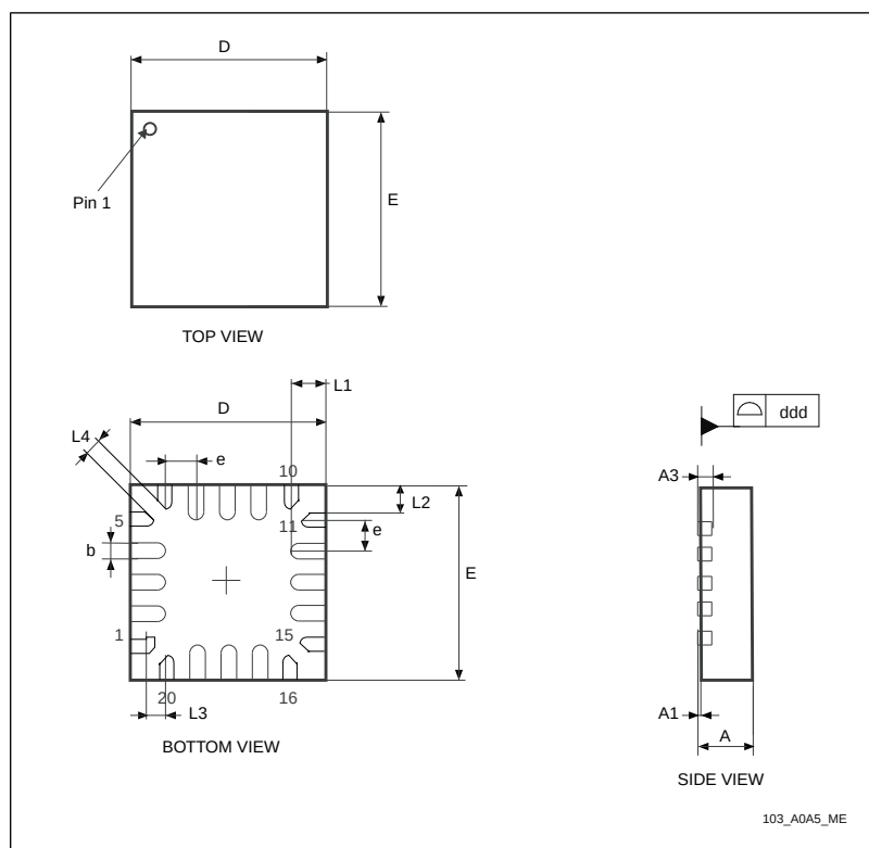
Figure 47: 20-lead, ultra thin, fine pitch quad flat no-lead package outline (3 x 3)
