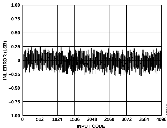
Figure 15. Typical AD5391-3 INL Plot
