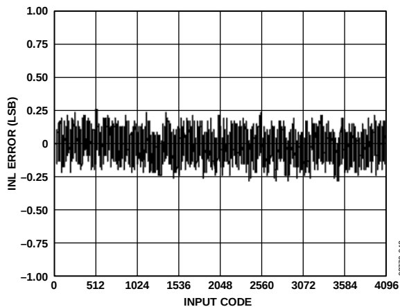
Figure 14. Typical AD5391-5 INL Plot
