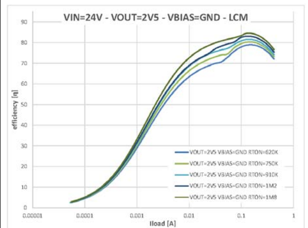
Figure 42. VIN 24 V - VOUT 2.5 V (log scale)
