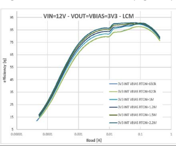
Figure 36. VIN 12 V - VOUT 3.3 V (log scale)
