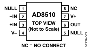
Figure 1. 8-Lead MSOP (RM Suffix)
