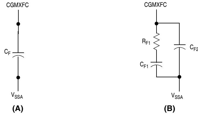
Figure 4-10. PLL Filter
