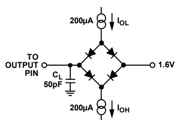
Figure 2. Load Circuit for Digital Output Timing Specifications
