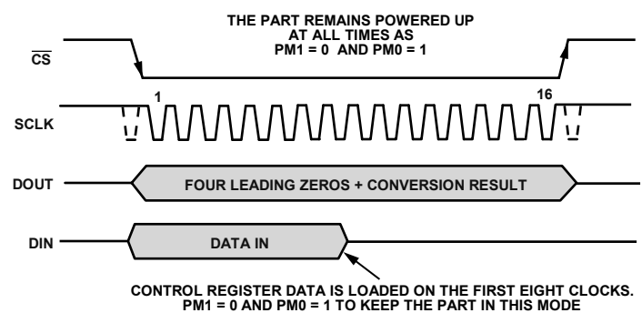
Figure 17. Mode 2 Operation
