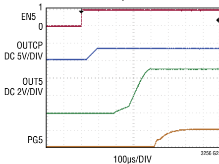
OUT5 Power-Up
