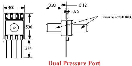
Dual Pressure Port
