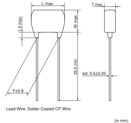
Dimensions code: 0 Lead style code: A2
