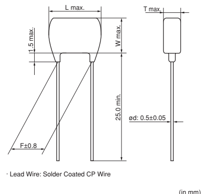
Dimensions code: 1 Lead style code: A2
