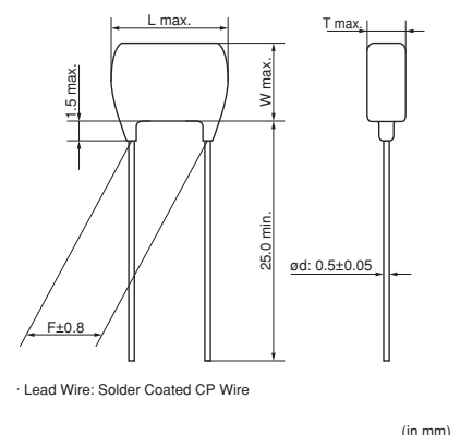
Dimensions code: 3 Lead style code: A2
