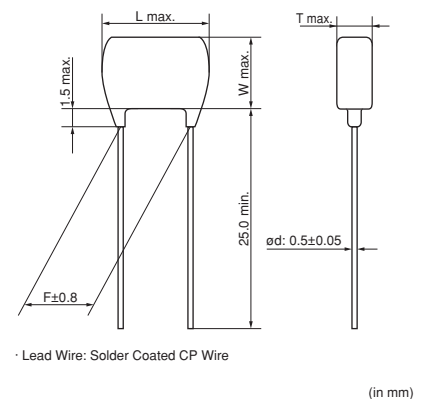
Dimensions code: 2 Lead style code: A2
