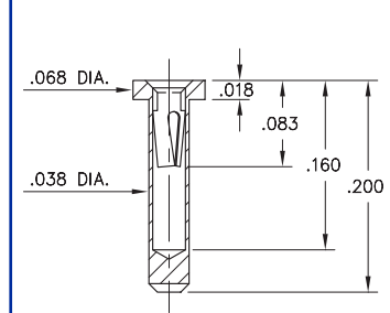
5552-0-15-XX-05-XX-10-0 Solder mount in .040 min. mounting hole
