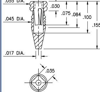
4994-0-15-15-11-27-10-0 Compliant press-fit in .041 - .044 Dia. mounting hole
