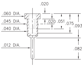
7491-0-15-XX-X1-XX-04-0 Press-fit in .042 mounting hole
