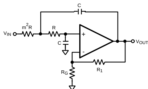
Figure 44. Sallen-Key Low Pass Filter
