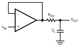
Figure 41. Compensation by Isolation Resistor
