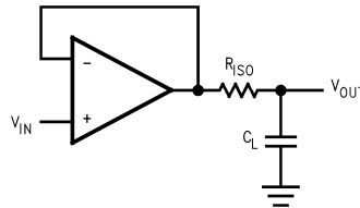
Figure 41. Compensation by Isolation Resistor
