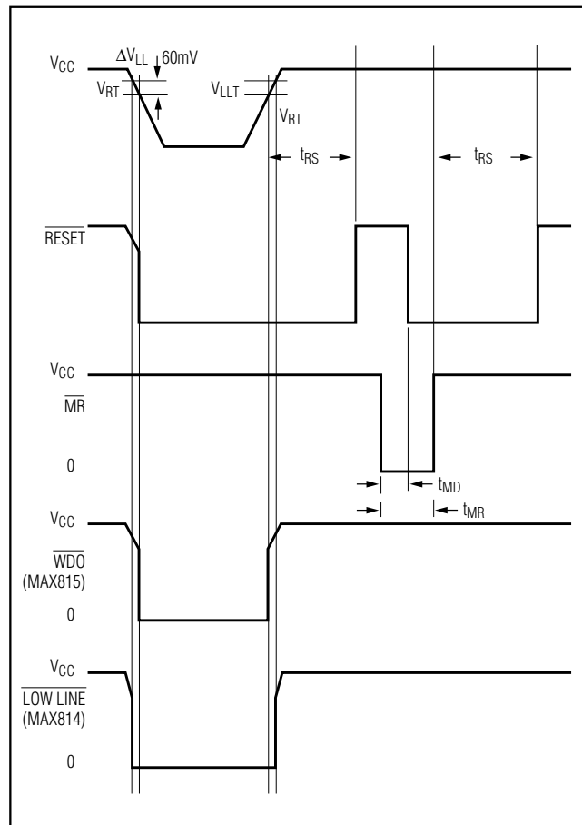
Figure 9. Timing Diagram
