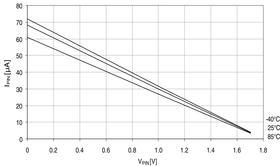
Figure 38-62. Reset pin pull-up resistor current vs. reset pin voltage. V_{CC} = 1.8V .
