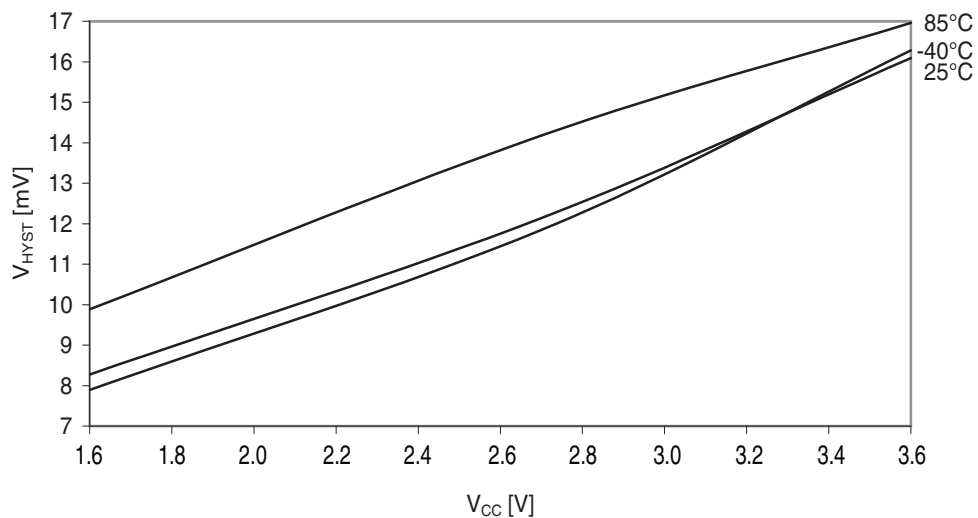
Figure 38-51. Analog comparator hysteresis vs. V_{CC} .
