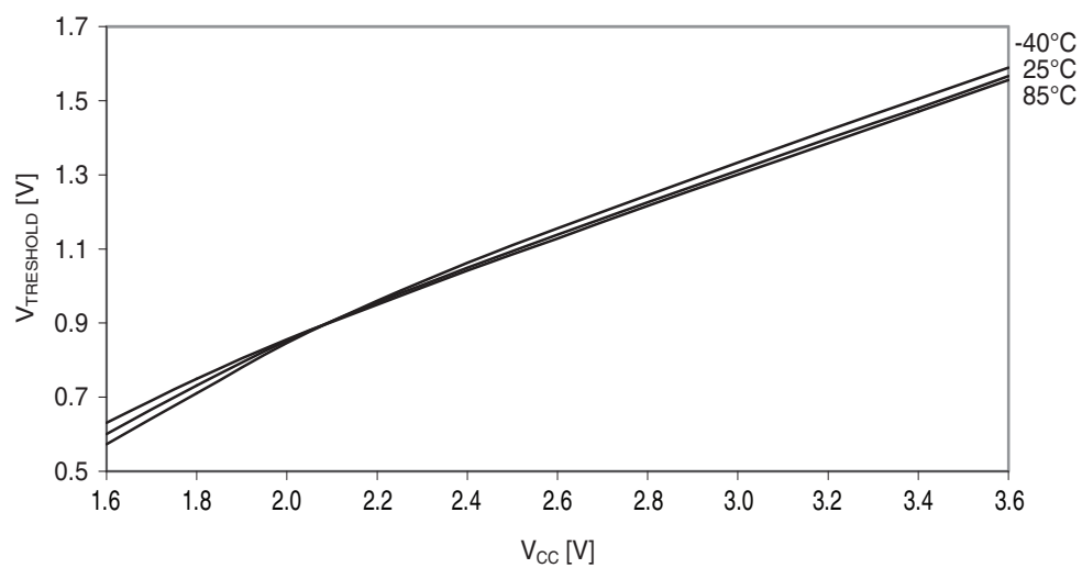
Figure 38-33. I/O pin input threshold voltage vs. V_{CC} . V_{IL} I/O pin read as "0".
