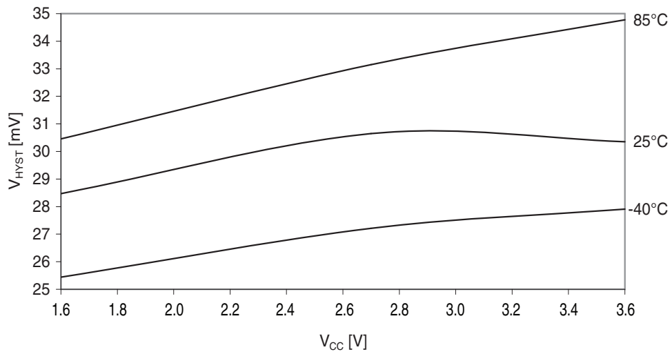
Figure 38-52. Analog comparator hysteresis vs. V_{CC} .
