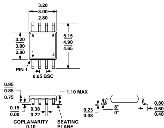
COMPLIANT TO JEDEC STANDARDS MO-187-AA Figure 61. 8-Lead Mini Small Outline Package [MSOP] (RM-8) Dimensions shown in millimeters
