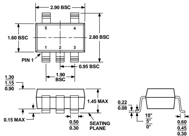
Figure 58. 5-Lead Small Outline Transistor Package [SOT-23] (RJ-5) Dimensions shown in millimeters
