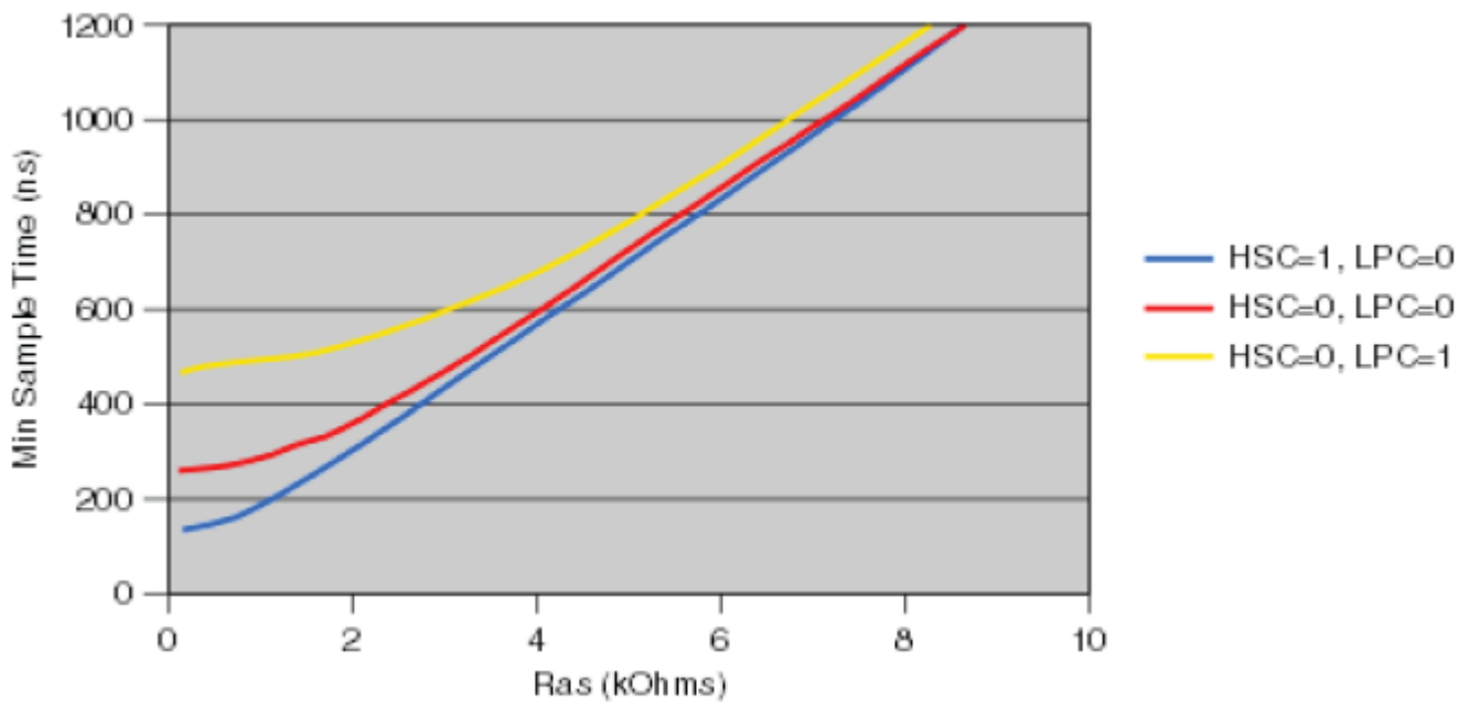
Figure 4-88. Minimum Sample Time Vs Ras (Cas = 10pF)
