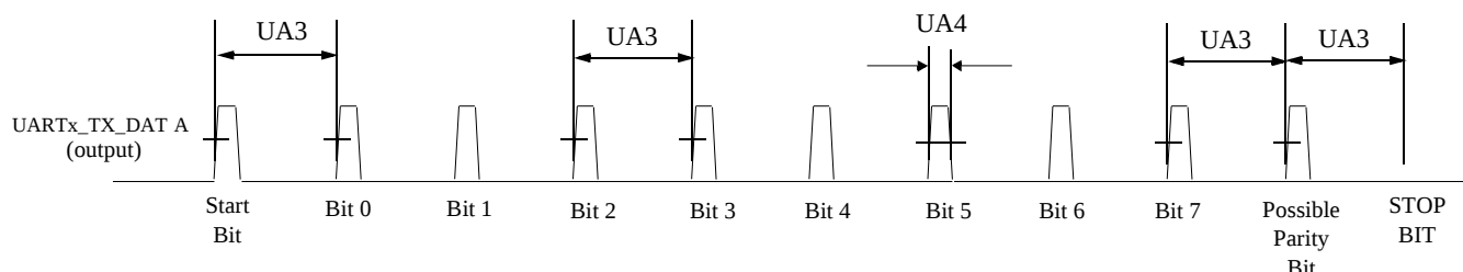
Figure 81. UART IrDA Mode Transmit Timing Diagram
