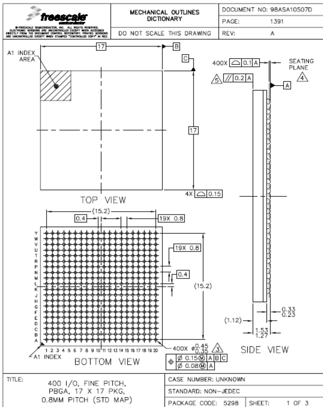
Figure 92. 17x17 mm BGA, Case x Package Top, Bottom, and Side Views
