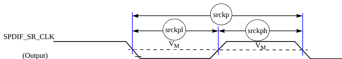
Figure 73. SPDIF_SR_CLK Timing Diagram
