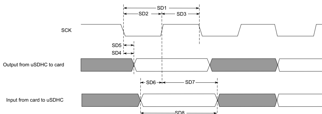
Figure 48. SDR50/SDR104 Timing
