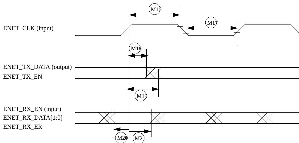
Figure 53. RMII Mode Signal Timing Diagram
