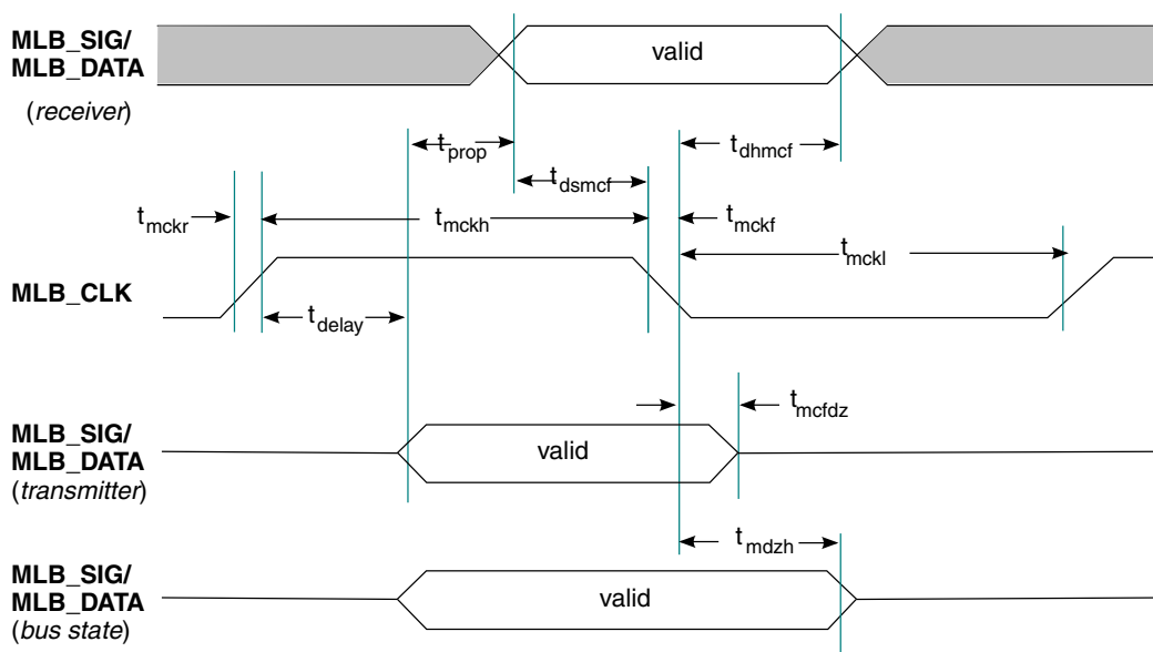
Figure 59. MediaLB 3-Pin Timing
