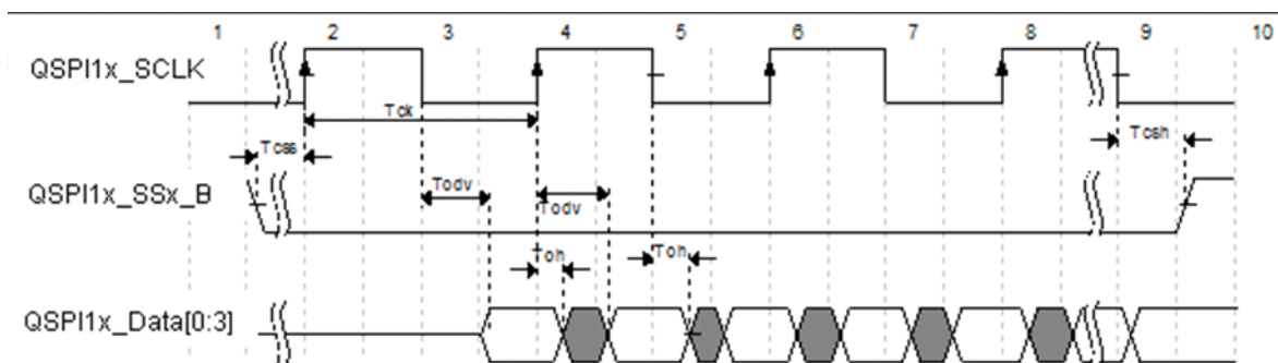
Figure 66. Figure 61. QuadSPI Output/Write Timing (DDR mode)
