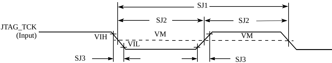
Figure 69. Test Clock Input Timing Diagram
