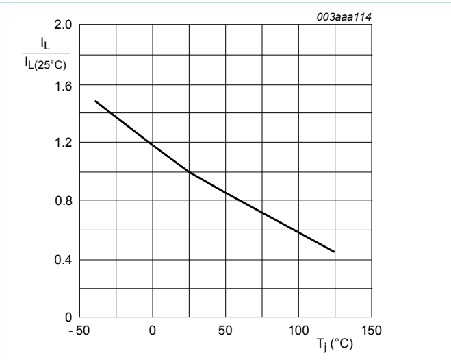
R_{GK} = 1 \text{ k}\Omega Fig. 8. Normalized latching current as a function of junction temperature
