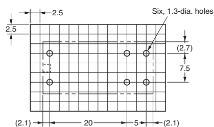
PCB Mounting Hole
