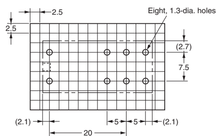
PCB Mounting Hole
