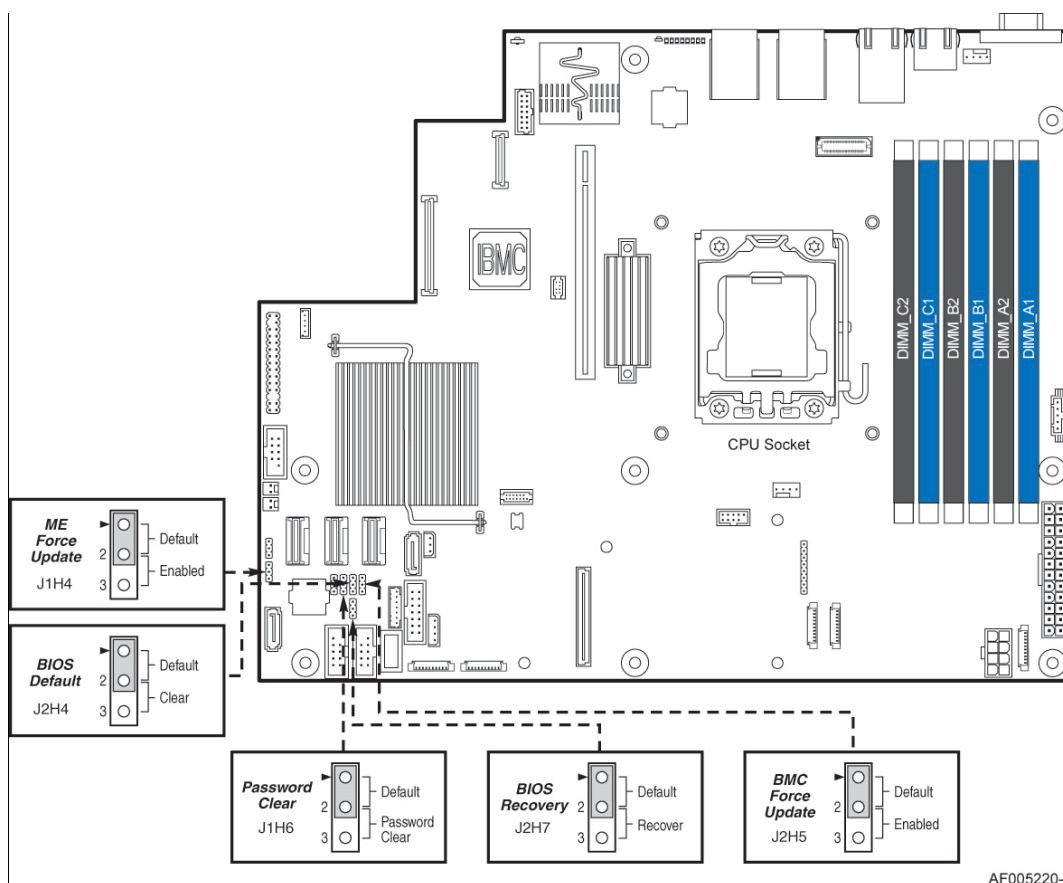
Figure 23. Jumper Blocks
