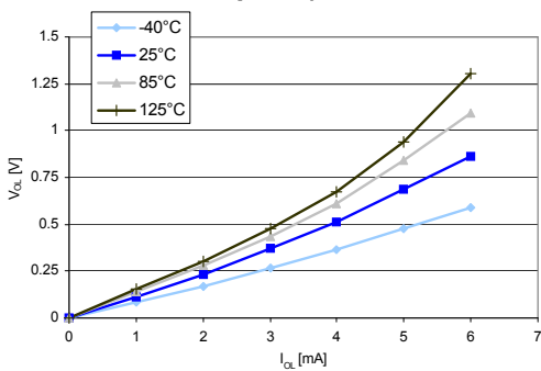
Figure 26. Typ. V_{OL} @ V_{DD} = 3.3 V (standard ports)
