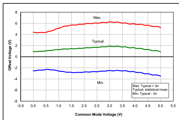
FIGURE 33-97: Op Amp, Offset over Common Mode Voltage, V_{DD} = 5.0V , T_{mp} = 25^\circ\text{C} PIC16F1704/8 Only.
