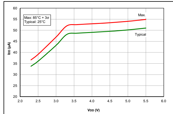
FIGURE 33-10: I_{DD} , EC Oscillator, Low-Power Mode, F_{OSC} = 500\text{ kHz} . PIC16LF1704/8 Only.
