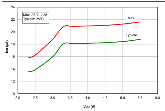
FIGURE 33-8: I_{DD} , EC Oscillator, Low-Power Mode, F_{OSC} = 32\text{ MHz} . PIC16LF1704/8 Only.
